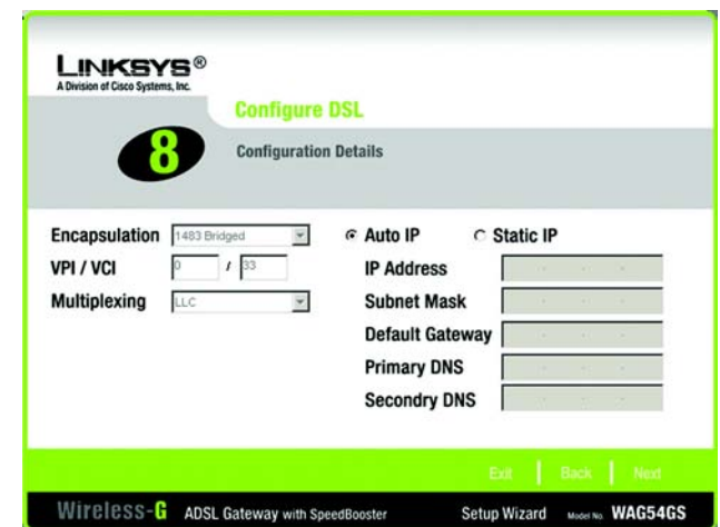
Figure 5-12: Setup Wizard's Configure DSL - 1483 Bridged Screen
